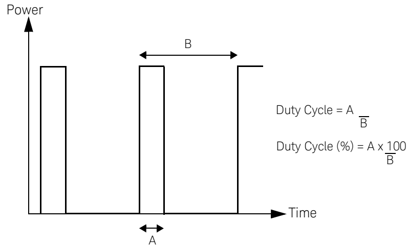
Figure 1-7 Pulsed signal
