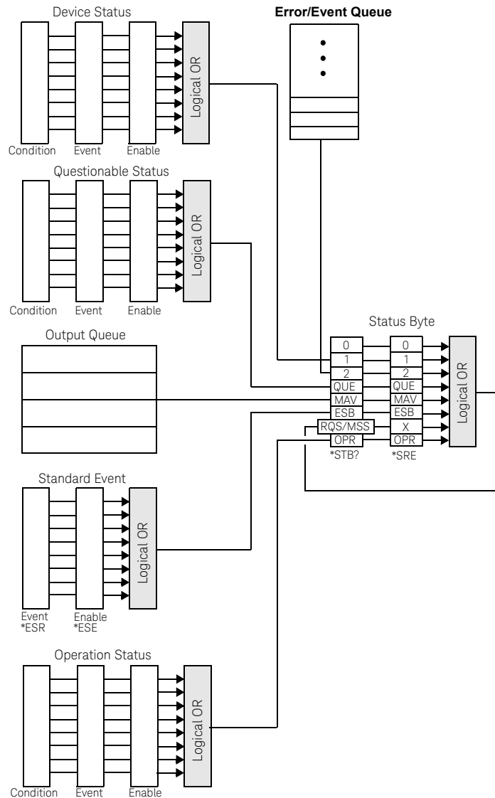
Figure 1-11 Status system
