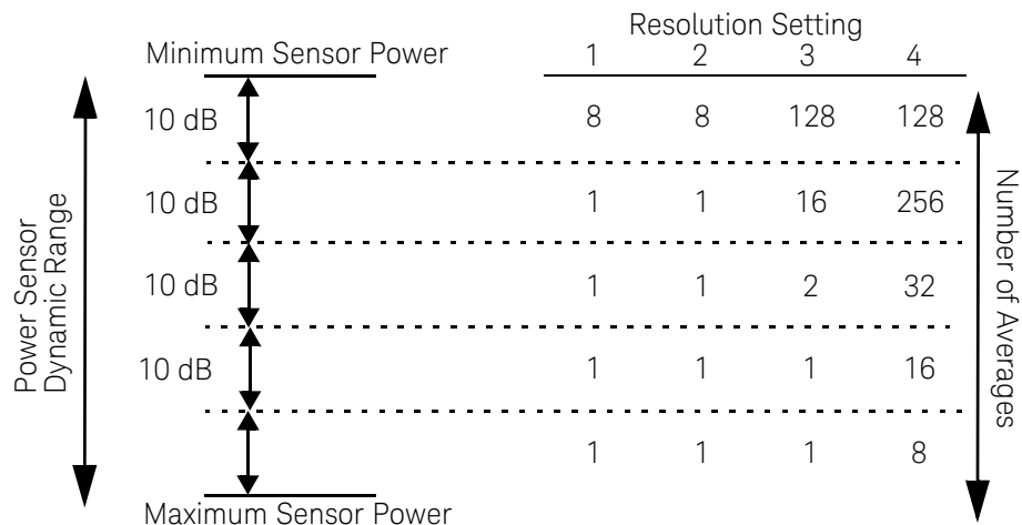
Figure 1-3 Averaged readings
