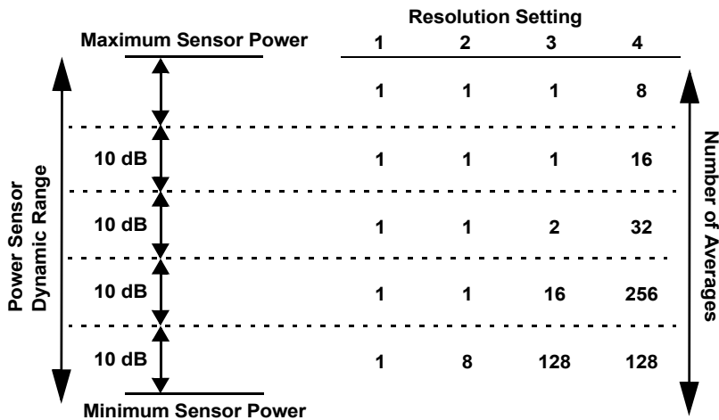
Figure 9-1 Average reading
