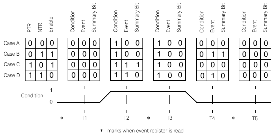
Figure 1-10 Typical status register bit changes
