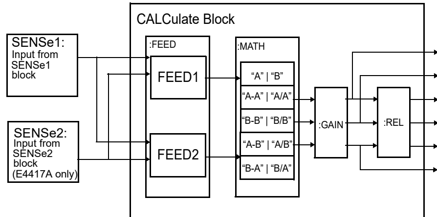
Figure 3-1 CALCulate block
