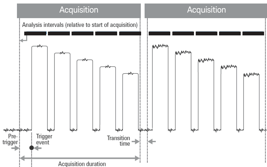
Figure 8. EXM's sequence capability with SAMM for DUT transmitter test
