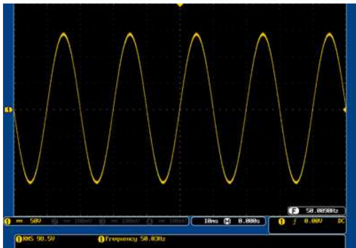
Sine waveform
