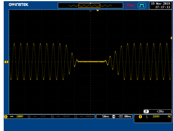
Power Outage
