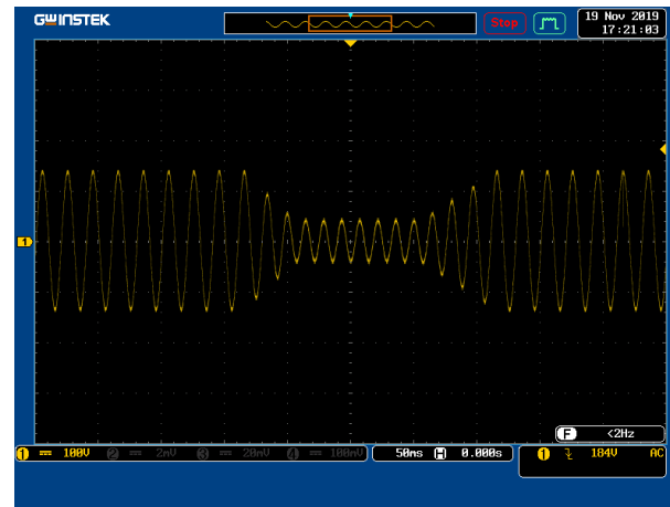
Voltage Fall
